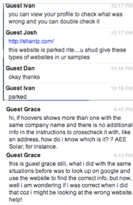
Figure 4. Worker-to-worker communication being used to clarify the user interface, the answer to a task, and the strategy used for solving it. Collaboration permits workers to debug tasks in situ and deal with unfamiliar tasks with managerial help without returning to requesters.
