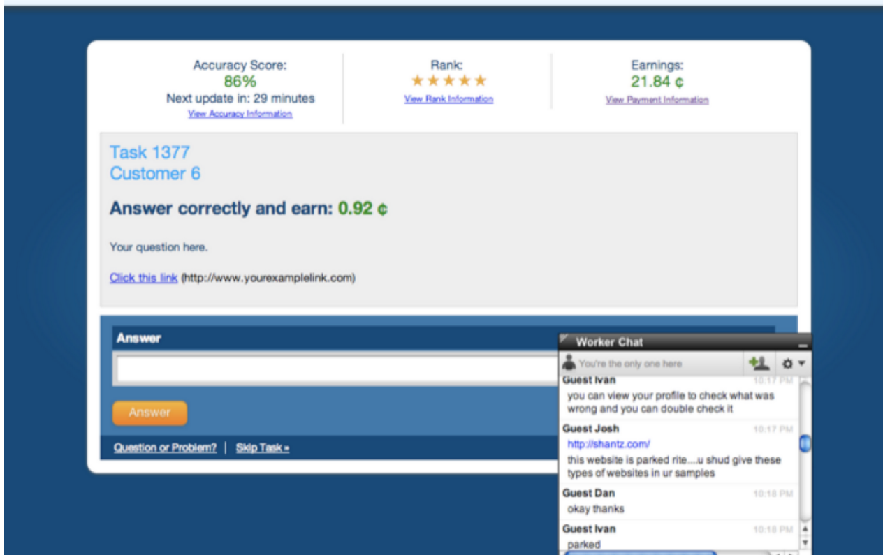
Figure 1. The MobileWorks interface serves a stream of appropriate tasks continuously to workers, interleaving qualification tests, expert tasks, unskilled tasks and training material. Workers are presented with immediate feedback on performance and earnings. Worker-to-worker chat is used to debug tasks on the fly, and workers can escalate tasks for managerial review.
